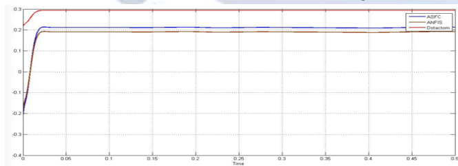
Case6: Reactive powers of modified D-statcom, ASFC and ANFIS ASFC when wind speed changes.
