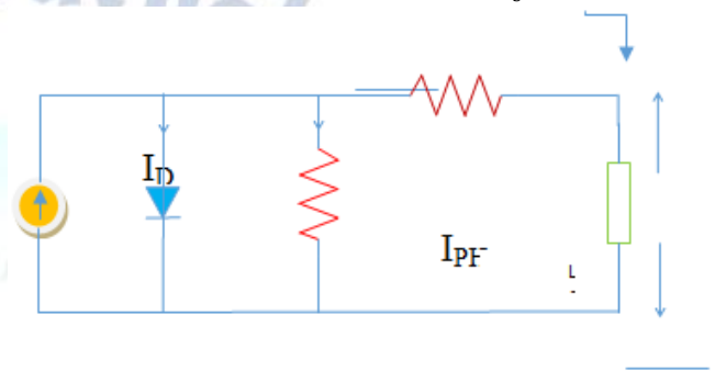
Fig. 2. PV Electrical Equivalent circuit
