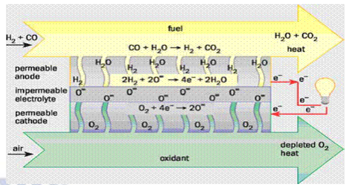
Fig 5: Operating principle of Fuel Cell
