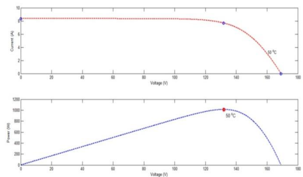
Fig. 3. Response of output characteristics of PV Array
