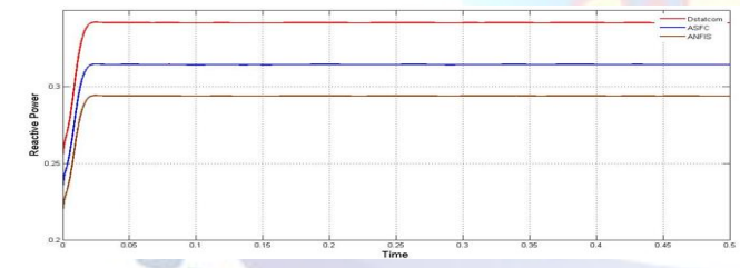
Case5: Reactive powers of modified D-statcom, ASFC and ANFIS ASFC when PV irradiation changes
