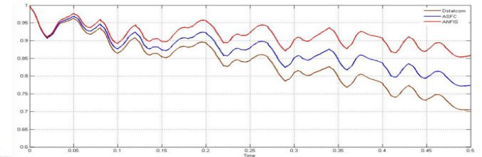
Case8: Power factors of modified D-statcom, ASFC, ANFIS ASFC when PV irradiation changes.
