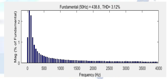
A.THDv of the voltage at the pcc using ASFC, modified D-statcom and ANFIS ASFC
