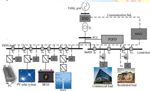
Figure 1: Diagram of an isolated MG with control system structure
