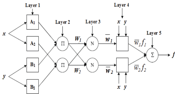
Fig 9 ANN architecture for a two-input multi-layer network
