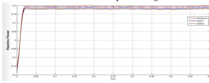
Case6: Reactive powers of modified D-statcom, ASFC and ANFIS ASFC when wind speed changes.
