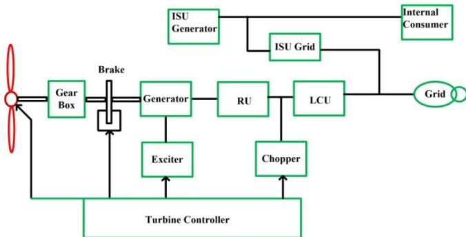
Fig. 4. Basic diagram of wind turbine
