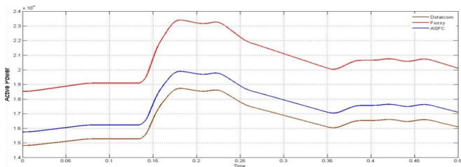
Case2: Active powers of modified D-statcom, ASFC and ANFIS ASFC when PV irradiation changes
