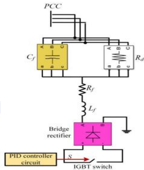
Figure 7: The proposed ASFC
