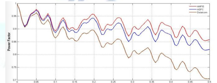
Case9: Power factor of modified D-statcom, ASFC, ANFIS ASFC when wind speed changes.
