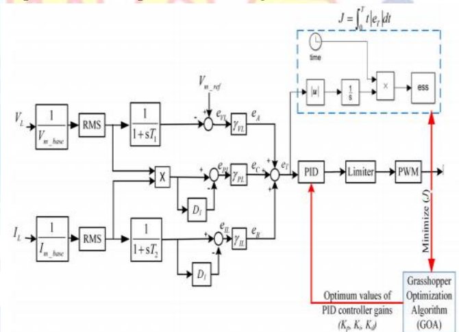
Figure 8: The PID controller using (GOA) with PWM circuit
