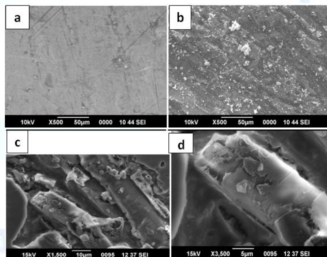
Figure 1 The SEM images of the morphologies of electrolysis product A
