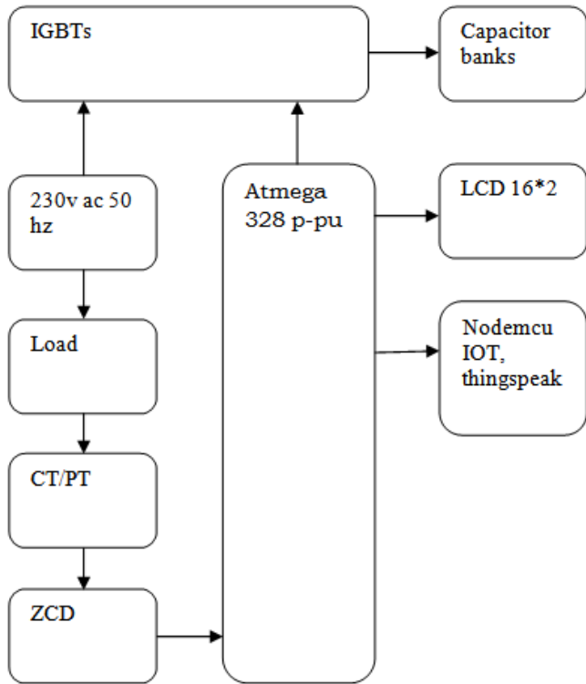
Figure1: Basic Block Diagram
