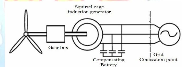
Figure 6: SCIG based WES
