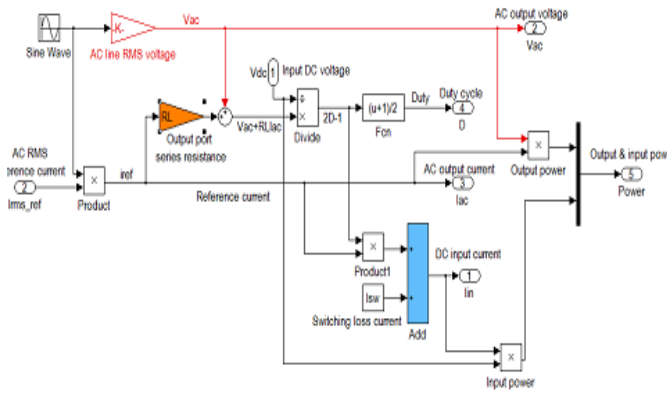
Figure 8: Control Diagram for Power management strategy in Hybrid System
