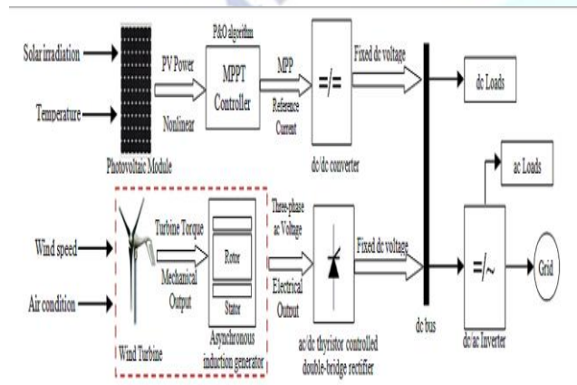
Fig 1: Basic architecture of Hybrid System
