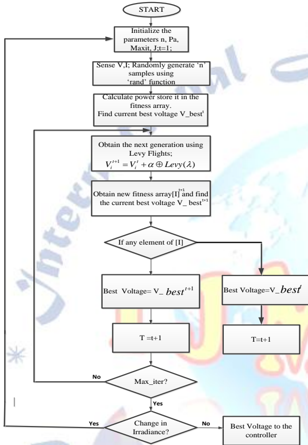
Figure 4: Cuckoo Search Algorithm
