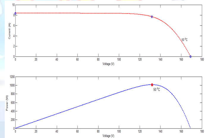
Figure 3: V-I Characteristics of PV system
