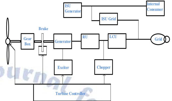
Figure 5: Basic Wind Turbine System
