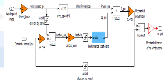
Figure 7: Implementation of Wind Turbine System
