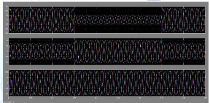
Fig.5. Insert Ultracapacitor Voltage for load maintained
