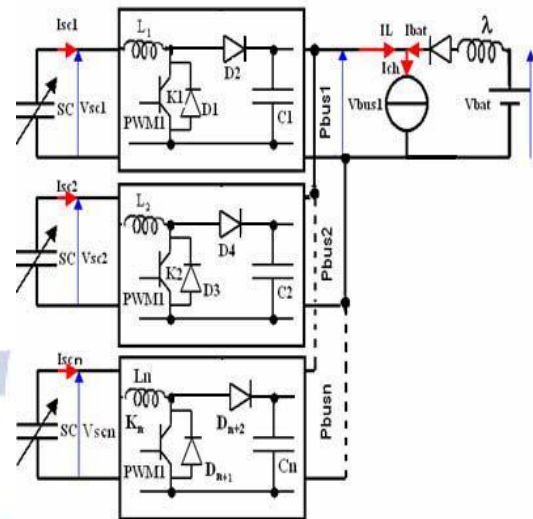
Fig 2(a): Multi boost Converter topology
