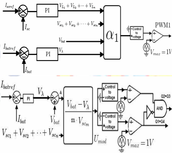
Fig 3. Multi boost and Multi full bridge converters control strategy
