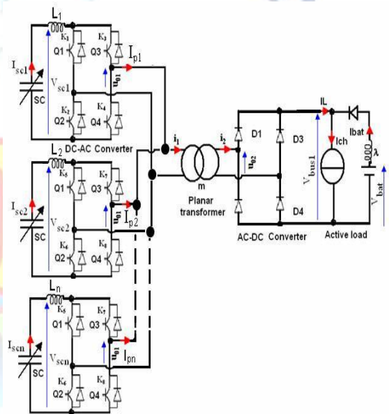
Fig 2(b): Multi full bridge converter topology
