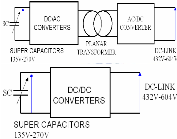
Fig1: Converter topologies for ECCE Hybrid Vehicle
