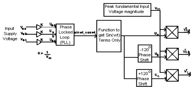
Fig 6 Extraction of Unit Vector Templates and 3-Ph Reference Voltages
