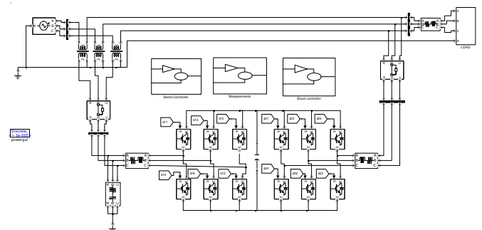
Fig 8 Matlab/Simulink Model
