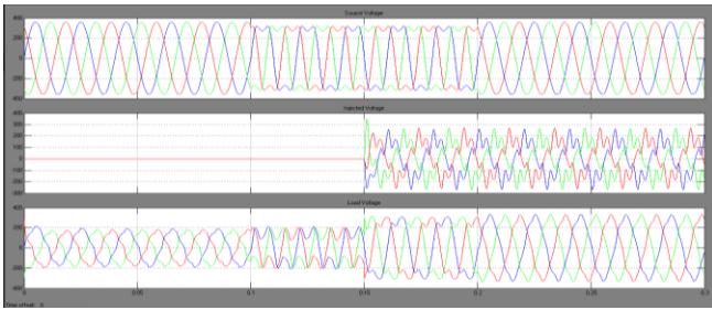
Fig 9 Simulation Results (a) Supply Voltage (b) Injected Voltage through Series Converter and (c) Load Voltage
