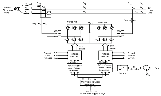
Fig 7 Overall Control Circuit Configuration of UPQC
