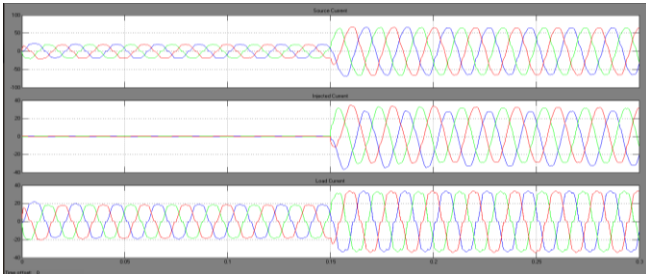
Fig 10 Simulation Results (a) Supply Current (b) Current at series converter and (c) Load Current
