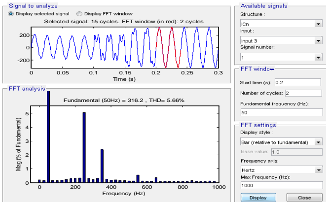
Fig 13 THD Analysis with UPQC (5.66%)
