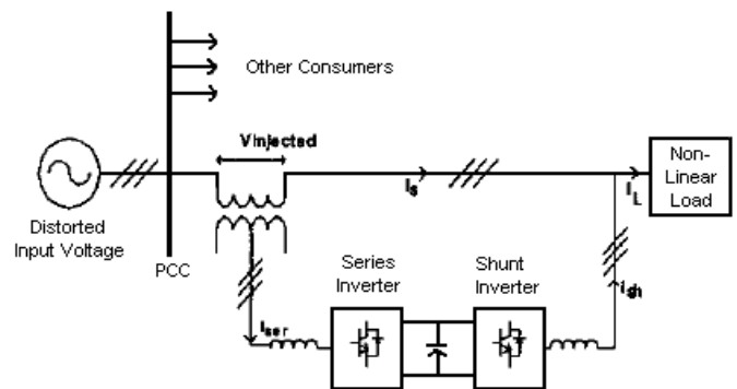
Fig 5 Basic Block Diagram of UPQC
