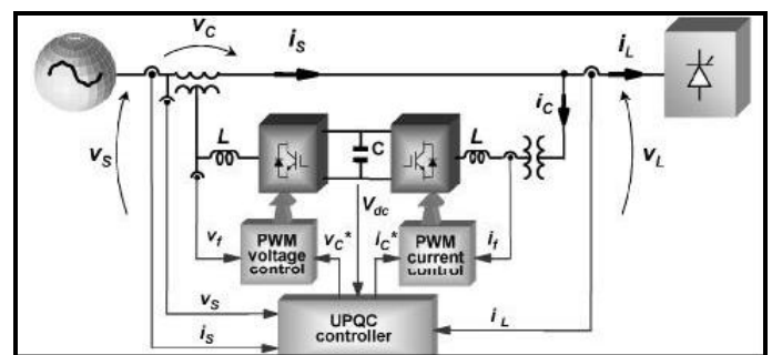
Fig: 4 Basic Configuration of the UPQC
