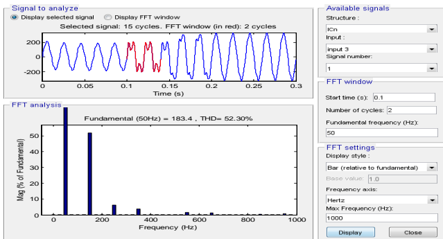
Fig 12 THD Analysis without UPQC (52.30%)
