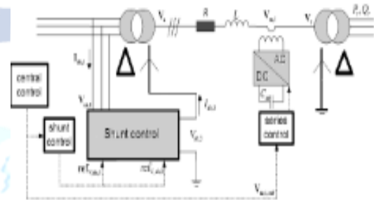
Fig 5: Structure of DPFC
