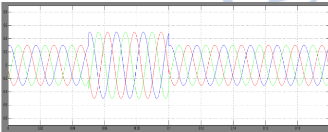
Fig 9: Simulation results for mitigation of current swell with DPFC system
