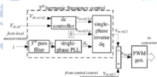
Fig 3: Block Diagram for Series Controller
