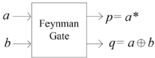
Figure 1. Feynman gate with target and garbage output.
