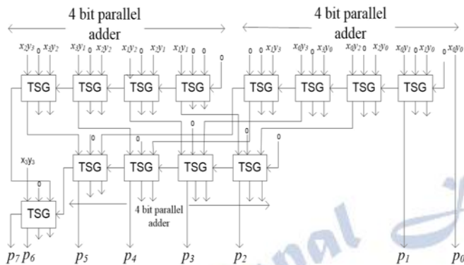
Figure 6. 4 \times 4 reversible Booth's multiplier [3].
