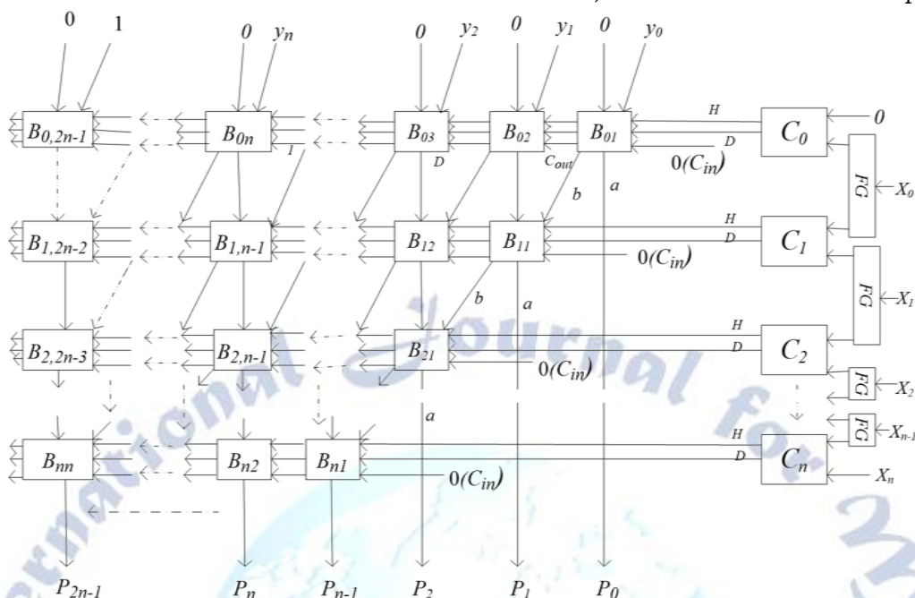
Figure 4. n \times n reversible Booth's multiplier.
