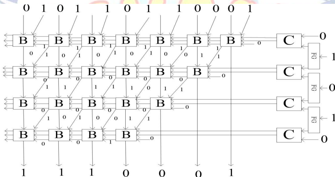
Figure 5. 4 \times 4 reversible Booth's multiplier.
