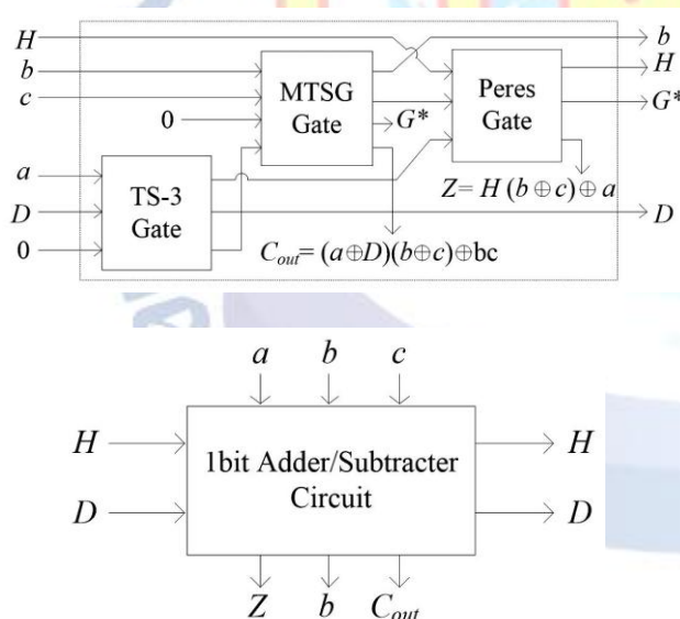
Figure 3. (a) Circuit diagram of B cell ( G^* indicates the garbage output) (b) Block diagram of B cell
