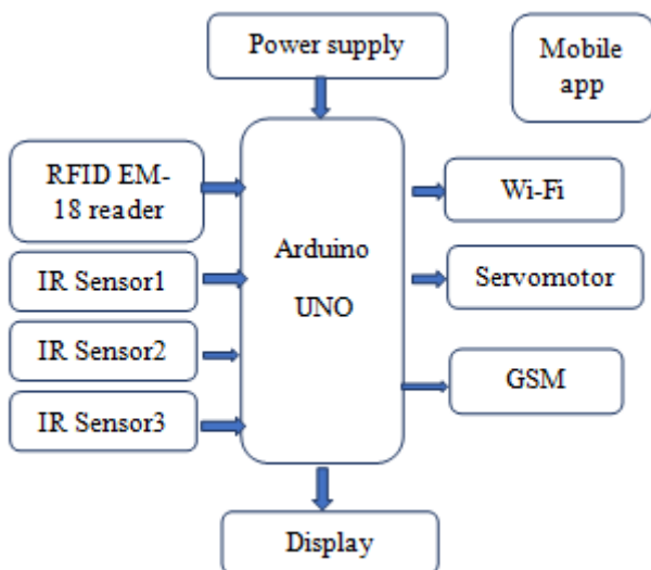
Fig.2 Block diagram for parking slot detection
