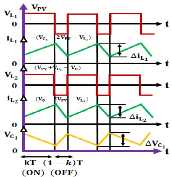
Figure 3 Re-lift Luo converter's voltage and current waveforms
