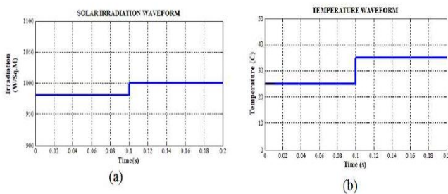
Figure 4 Waveforms of (a) Solar irradiation and (b) Temperature
