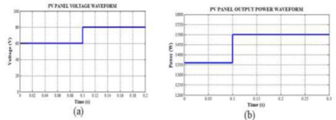
Figure 5 (a) Waveforms of PV panel voltage and (b) PV panel output power
