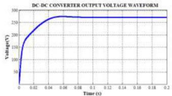
Figure 6 Re-lift Luo converter voltage output waveform
