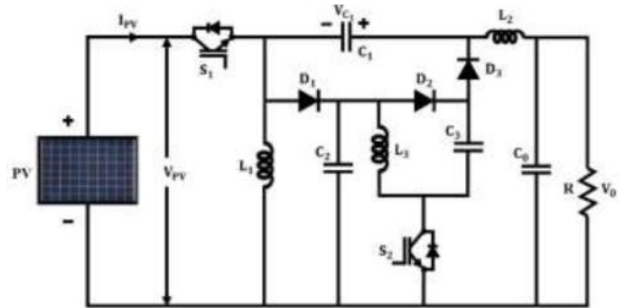
Figure 2 Circuit diagram of re-lift converter
