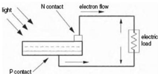
Fig 2.1: PV converts the photon energy into voltage across the p-n junction
