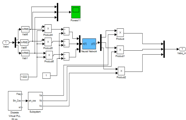
Fig 5.6 Inverter control with ANN control
