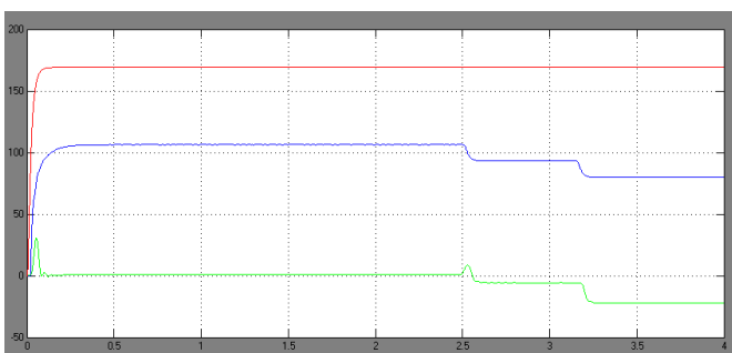
Fig 5.7 Simulation result with ANN control
