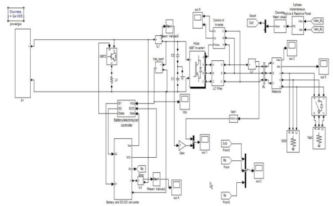
Fig.5.1 Proposed Model
