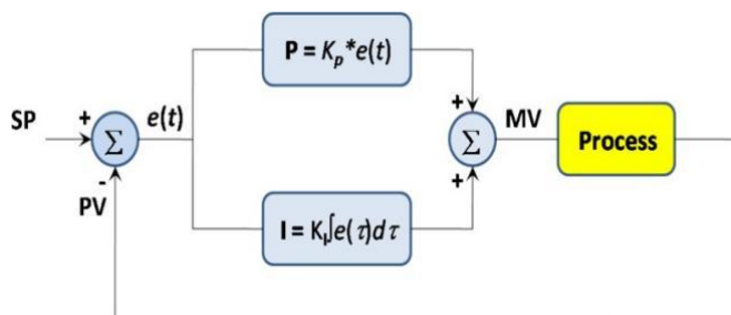
Fig.3.1: Block diagram of a PI controller
