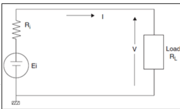
Fig 2.3: Equivalent electrical circuit of a Battery
