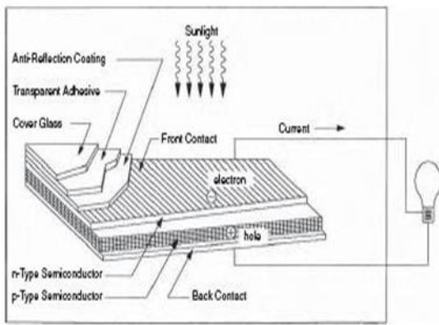
Fig 2.2: Basic construction of PV cell
