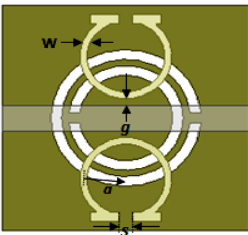
Fig.2 Schematic view of microstrip line loaded with Omega SRR coupled with SRR etched on a dielectric substrate
