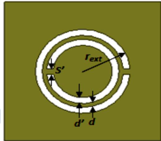
Fig.3 Schematic view of bottom surface of the CSRR etched on the ground plane
