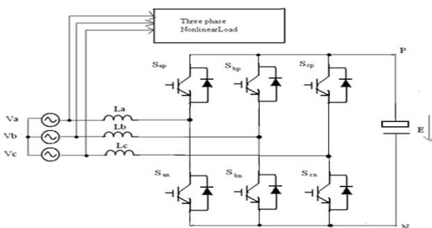
Fig.1 Power stage of the three-phase APF
