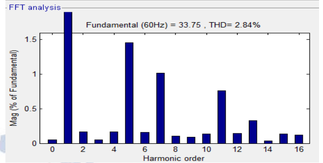
Fig.13 THD with fuzzy one cycle controller
