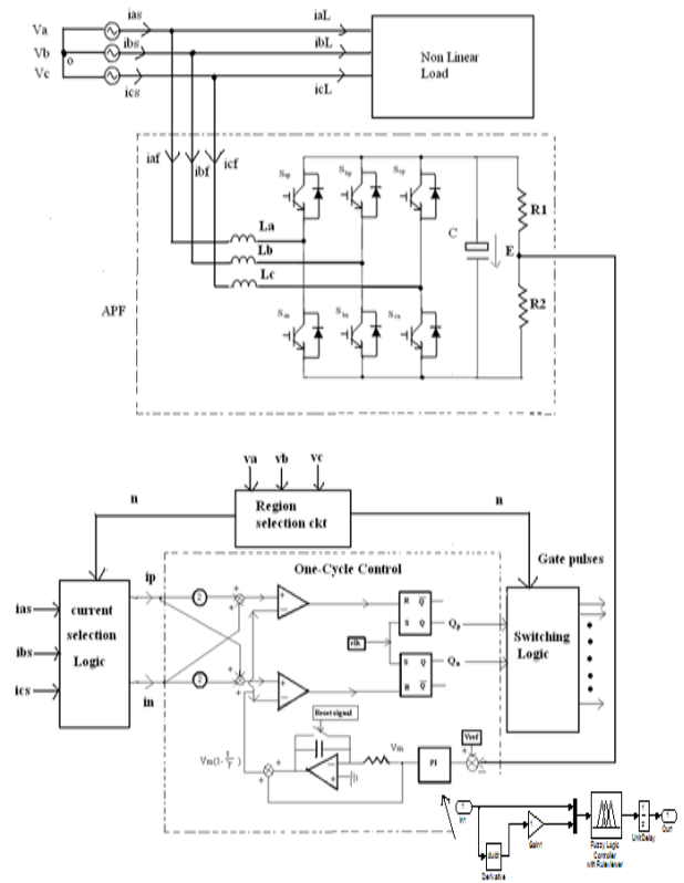
Fig.7 Block diagram of One-Cycle controlled APF with PI and Fuzzy controllers
