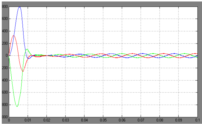
Fig.10 Source current with PI One cycle control
