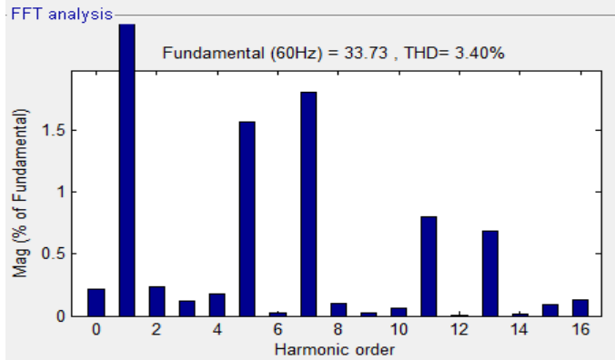
Fig.11 THD with PI One cycle controller
