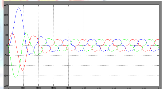
Fig.8 Source current without APF
