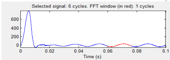
Fig.10 Source current with PI One cycle control
