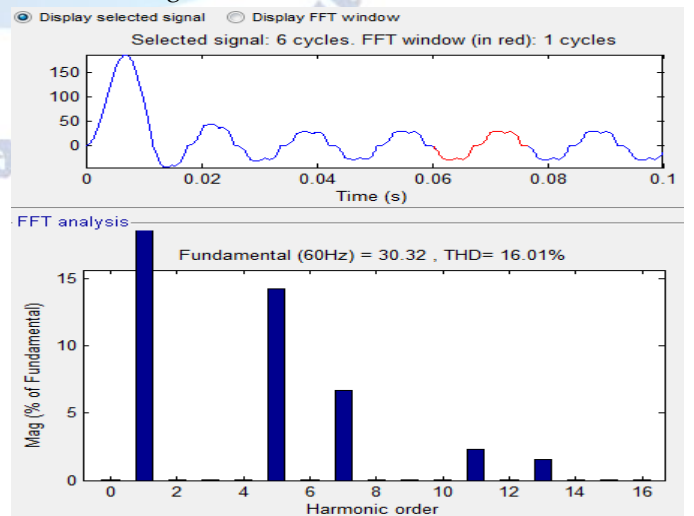
Fig.8 Source current without APF
