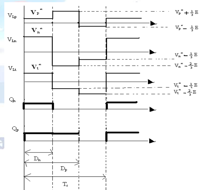
Fig.4 Inductor voltage waveforms for the converter under the condition d_p > d_n
