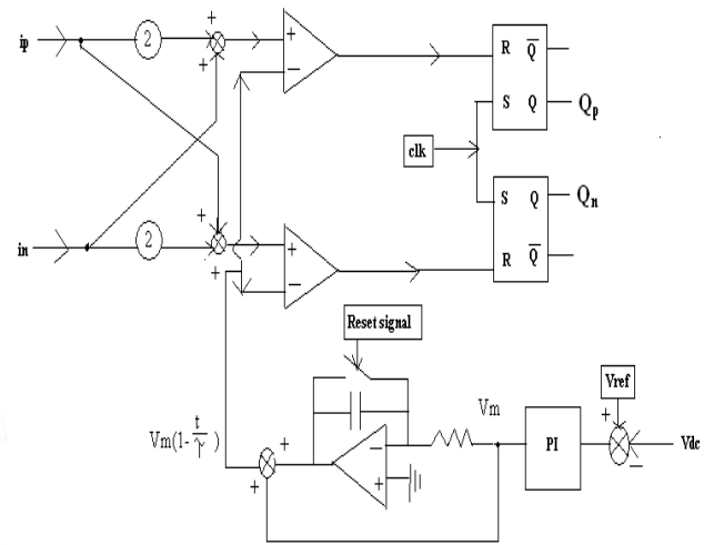
Fig.5 One- cycle control logic
