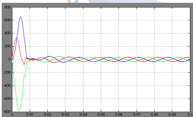
Fig.12 Source current with fuzzy one cycle control
