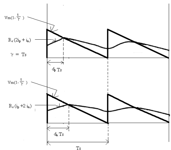
Fig.6 Operation waveforms of One-cycle controlled APF controller
