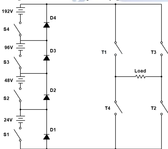
Fig. 3. Circuit Diagram
