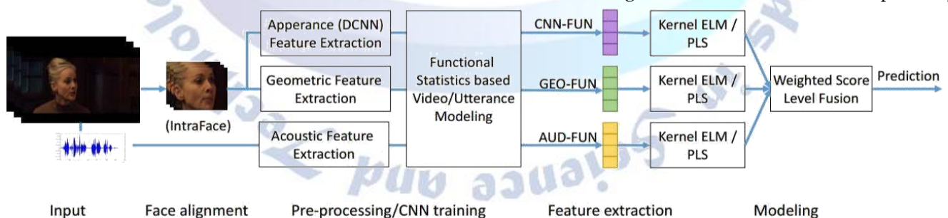
Fig.1. Audio-visual processing pipeline for Bipolar Disorder classification from vid
