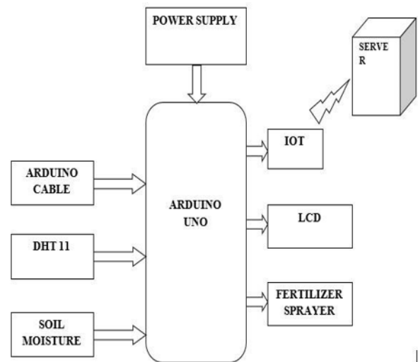
Fig-6: Hardware Block
