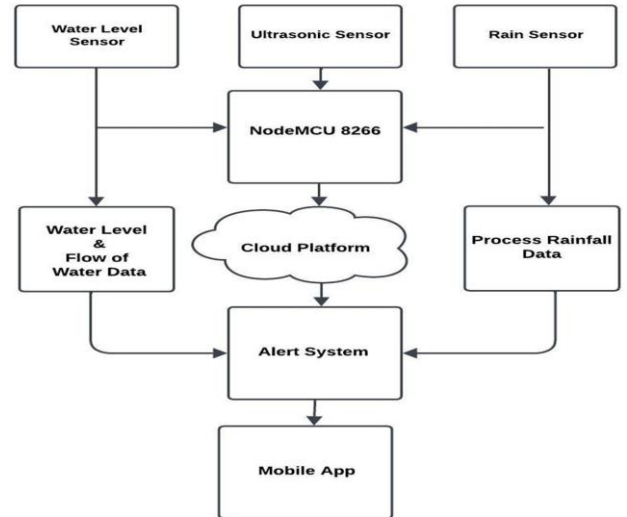
Fig. 2. Block Diagram of Flood Monitoring and Detection System [12]
