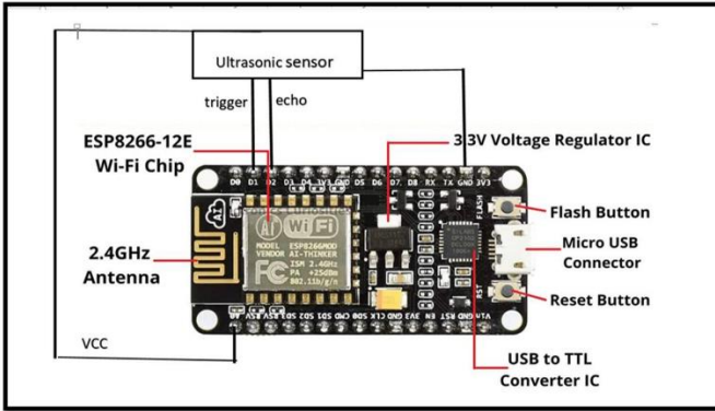
Fig. 1 Circuit Diagram of the ESP8266-12E-Based IoT Flood Monitoring System [9]
