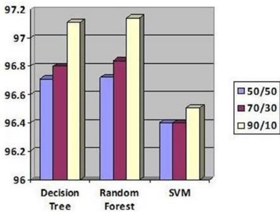
Fig. 1 Detection accuracy comparison
