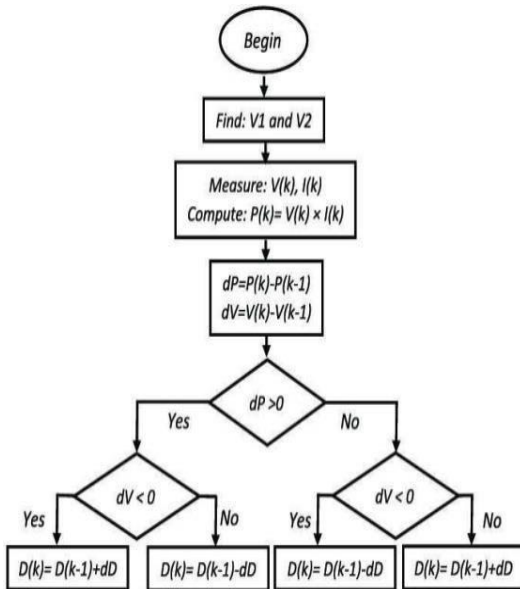
Fig. 6: Perturb and Observe Algorithm Flow Chart
