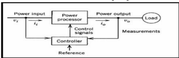
Fig. 4: Block diagram of a power electronic system
