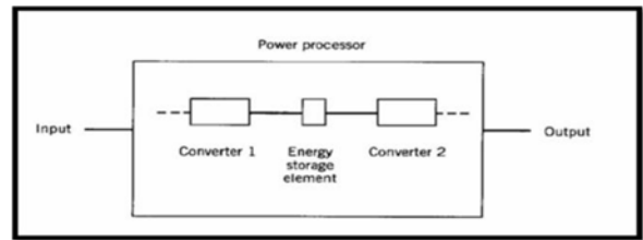
Fig. 5: Block diagram of a power processor.
