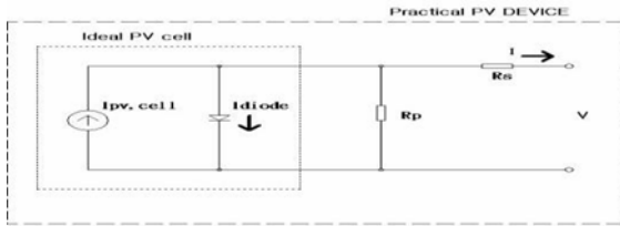
a) Fig.3: Equivalent model of a photovoltaic cell.
