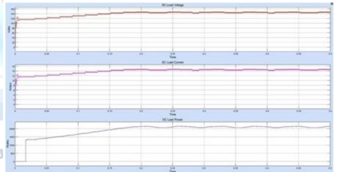
Fig. 8: Output wave forms of online MPPT technique (Perturb and Observe).
