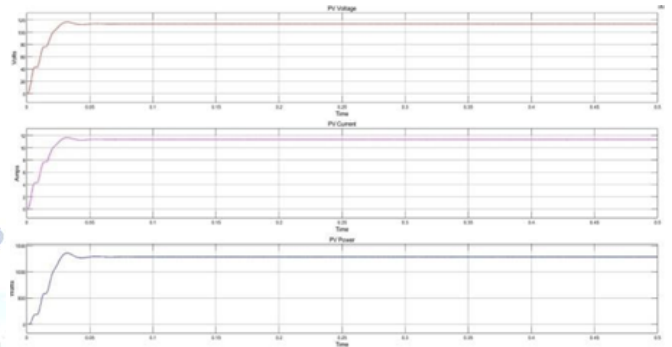
Fig. 7: Output wave forms of offline MPPT technique (OCV).
