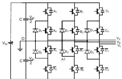
Fig.3. Three Level Inverter
