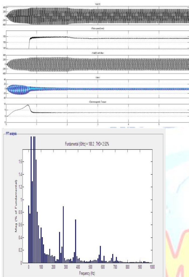
Fig.7. Variation of speed of the motor with change in irradiation Fig.8. THD analysis.
