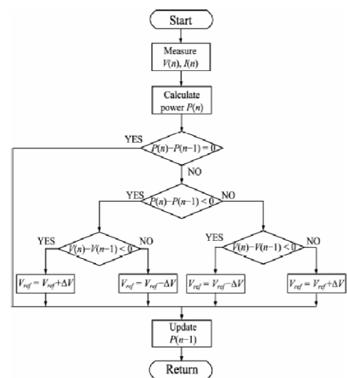
Fig.2. Flow chart of P&O Method
