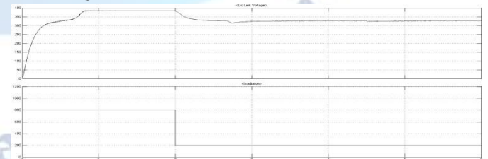
Fig.6. Change in dc link voltage with respect to irradiation.
