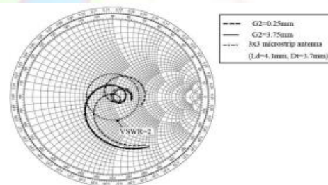
Figure 2. Impedance loci of one 3 \times 3 array and two 5 \times 5 arrays.
