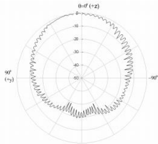
Figure 5. Measured spinning linear radiation pattern in yz -plane for the 5 \times 5 microstrip array at the center frequency.
