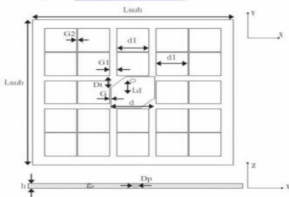
Figure 1. Geometry of a 5 \times 5 microstrip patch array.
