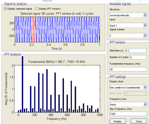
Figure 3: THD analysis 19.44% without LC filter
