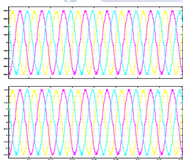
Figure 4: Voltage and current waveform using LC filter
