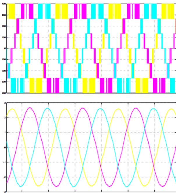
Figure 2: Voltage and current waveforms without LC filter
