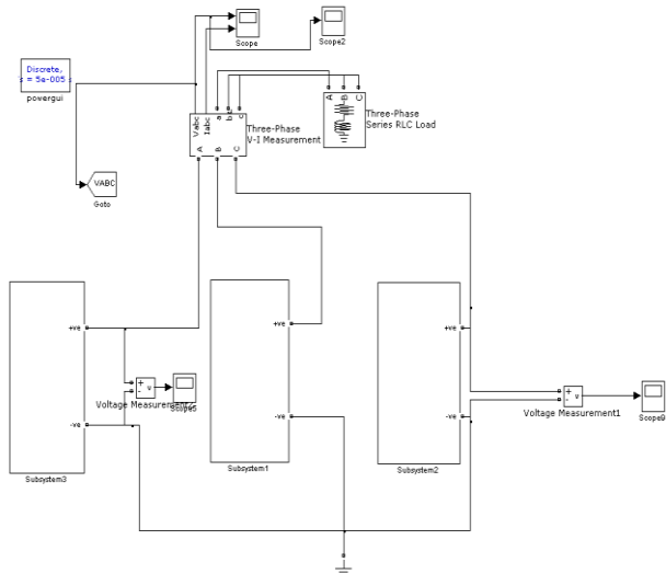
Figure 1: Matlab simulink main diagram
