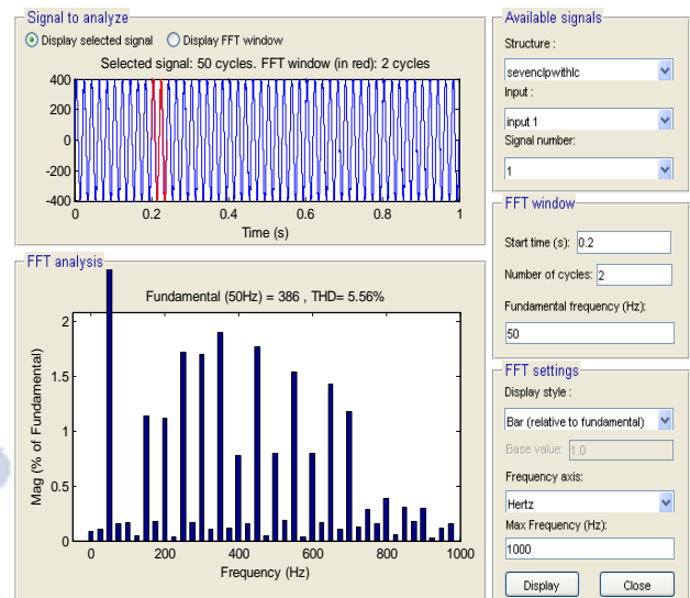
Figure 5: THD analysis 5.56% with LC filter
